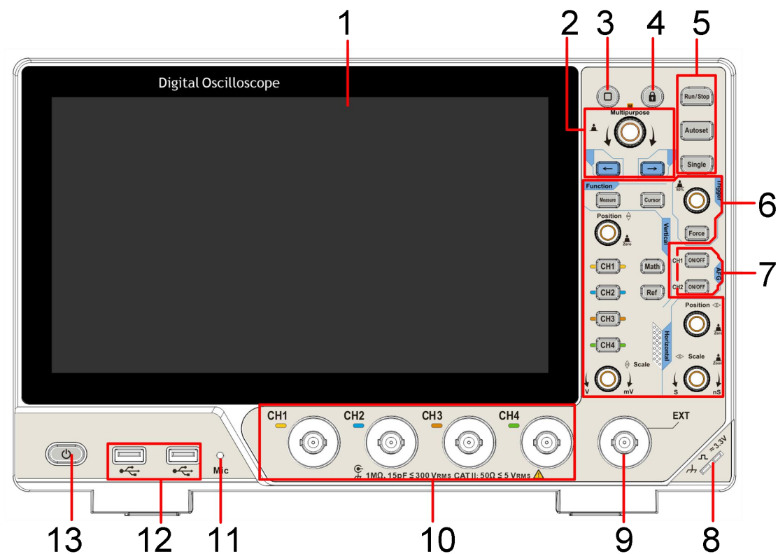
Figure 3-1: Front panel
