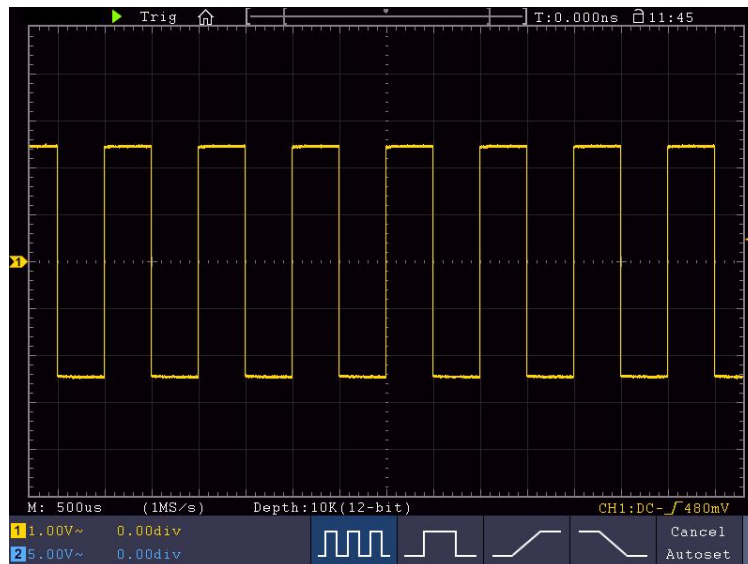
Figure 3-6 Auto set
