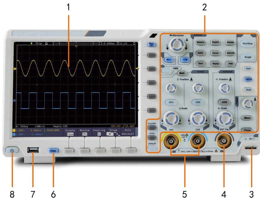
Figure 3- 1 Front panel
