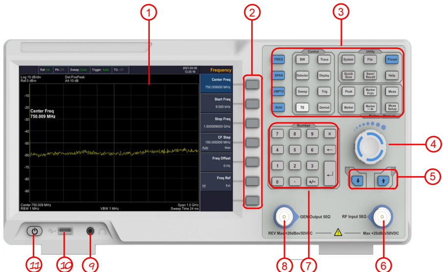
Figure 3- 1 Front panel
