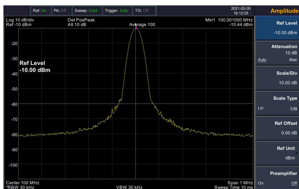
Figure 3- 10 Set reference level
