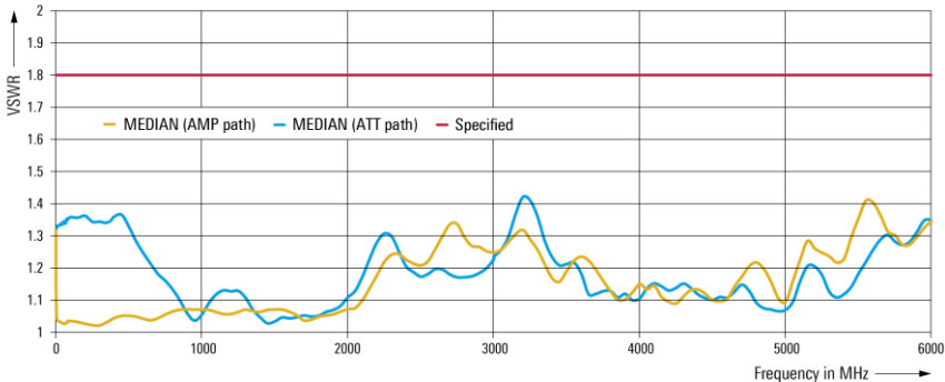
VSWR versus frequency (without R&S®SMBB-B32 option)
