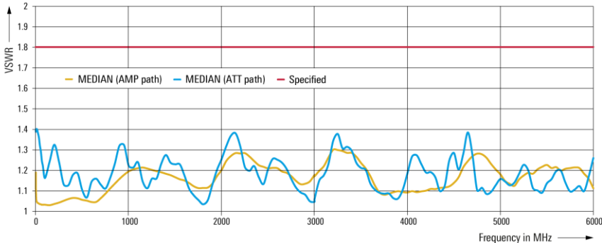
VSWR versus frequency (with R&S®SMBB-B32 option)
