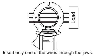
Insert only one of the wires through the jaws.
