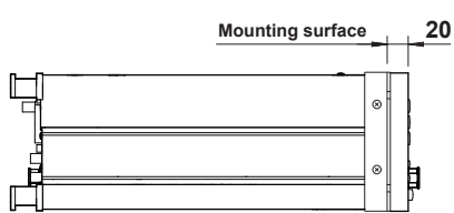
EIA rack mount dimensions
