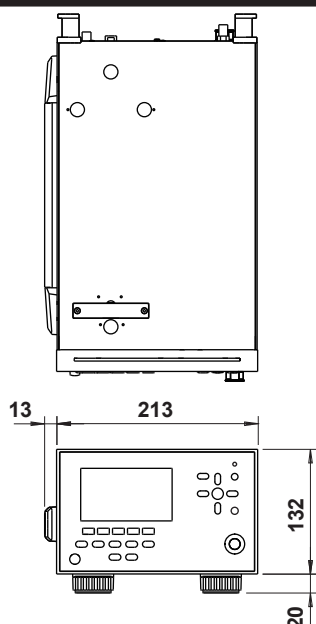
JIS rack mount dimensions
