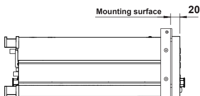
JIS rack mount dimensions
